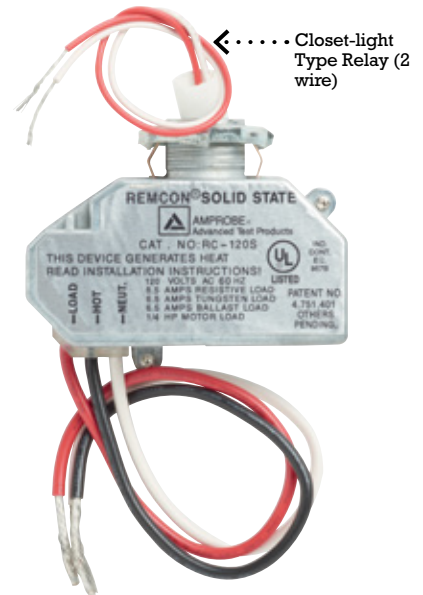
RC-120S Closet-light Type Relay
