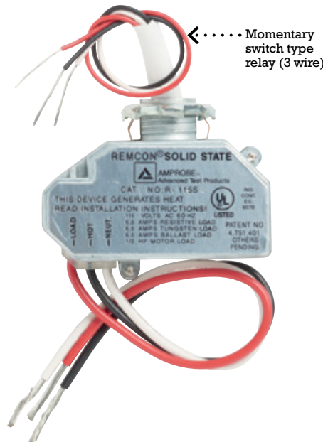
R-115S Momentary Switch Type Relay
